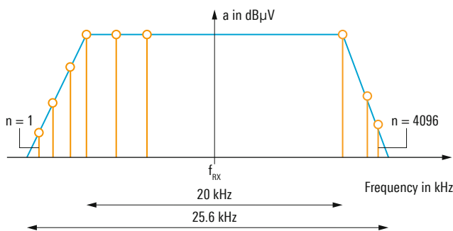
Actual sampling bandwidth compared with selected IF bandwidth
